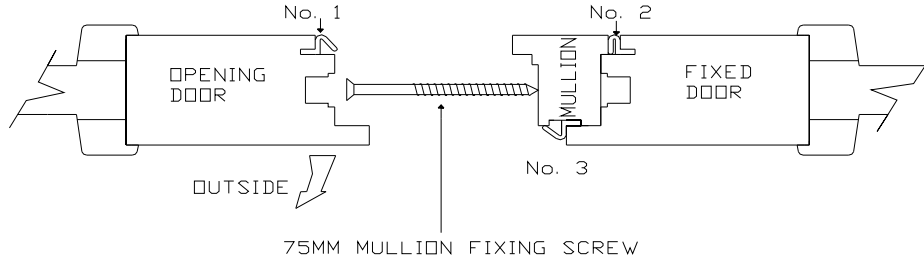
OPTION 2. OPENING OUT, RIGHTHAND DOOR OPENING
