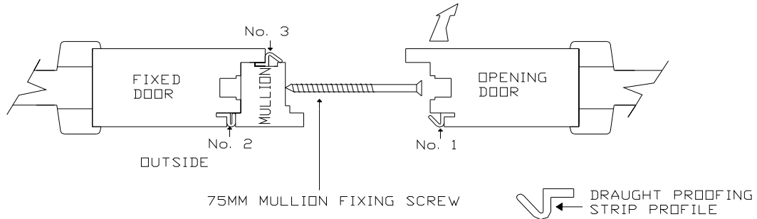
OPTION 4. OPENING IN, RIGHT HAND DOOR OPENING
