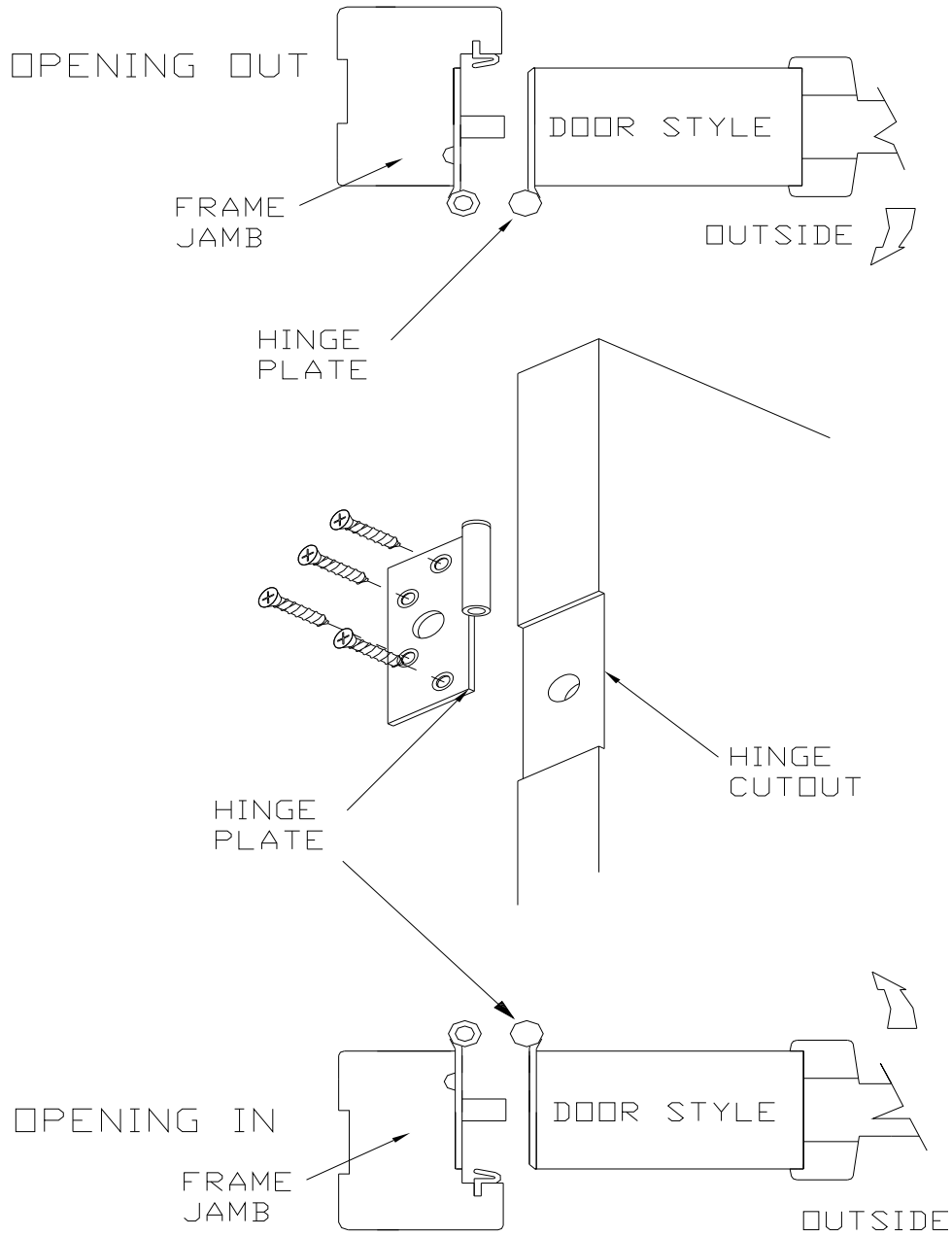
DIAGRAM 8 PLAN VIEW
