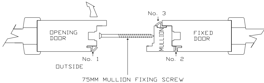
OPTION 3. OPENING IN, LEFTHAND DOOR OPENING
