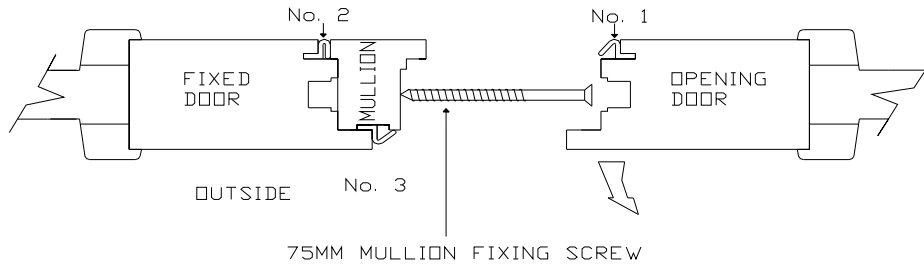
OPTION 2. OPENING OUT, RIGHTHAND DOOR OPENING
